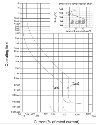
Operating time characteristics curve (Ambient temperature 30°C) (6A~63A)
