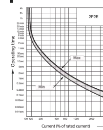
Operating characteristics curves (with O.C.)
